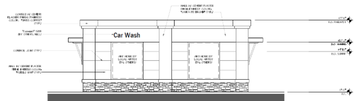
WEST CARWASH BUILDING ELEVATION (FACING UNIVERSITY AVE.) Scale: 1/8" = 1'-0"
