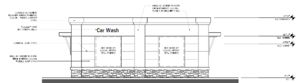
WEST CARWASH BUILDING ELEVATION (FACING UNIVERSITY AVE.)
