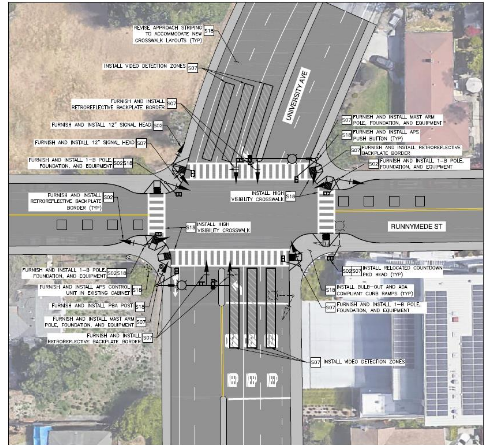
PROPOSED CONDITIONS
