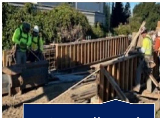
Wingwall Work
