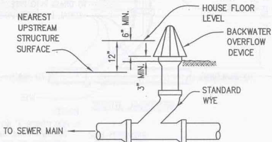
OVERFLOW SYSTEM
