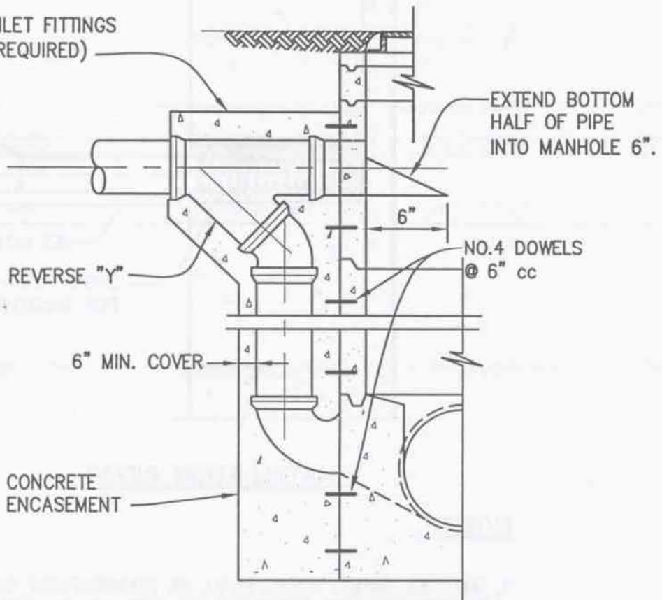
MANHOLES WITH DROP INLET
