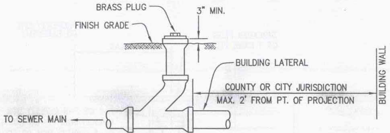
STANDARD CLEANOUT AT BUILDING UNIT
