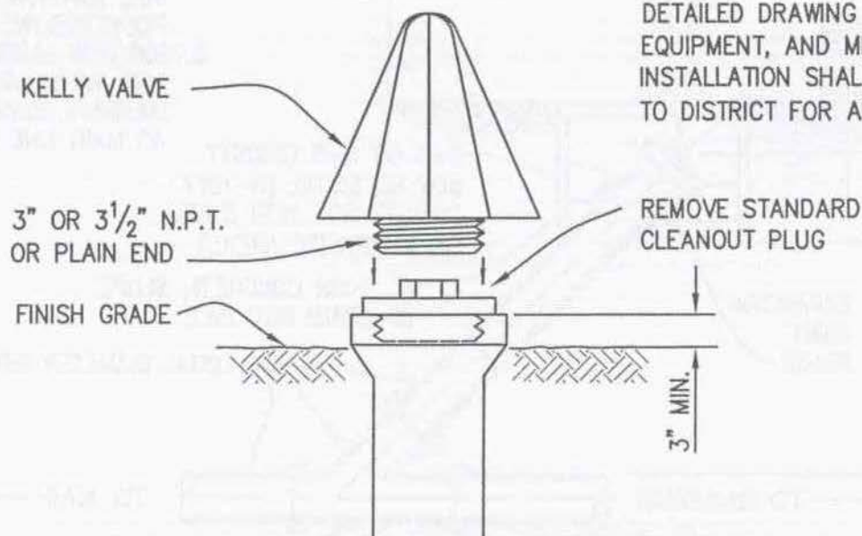
BACKWATER OVERFLOW DEVICE
