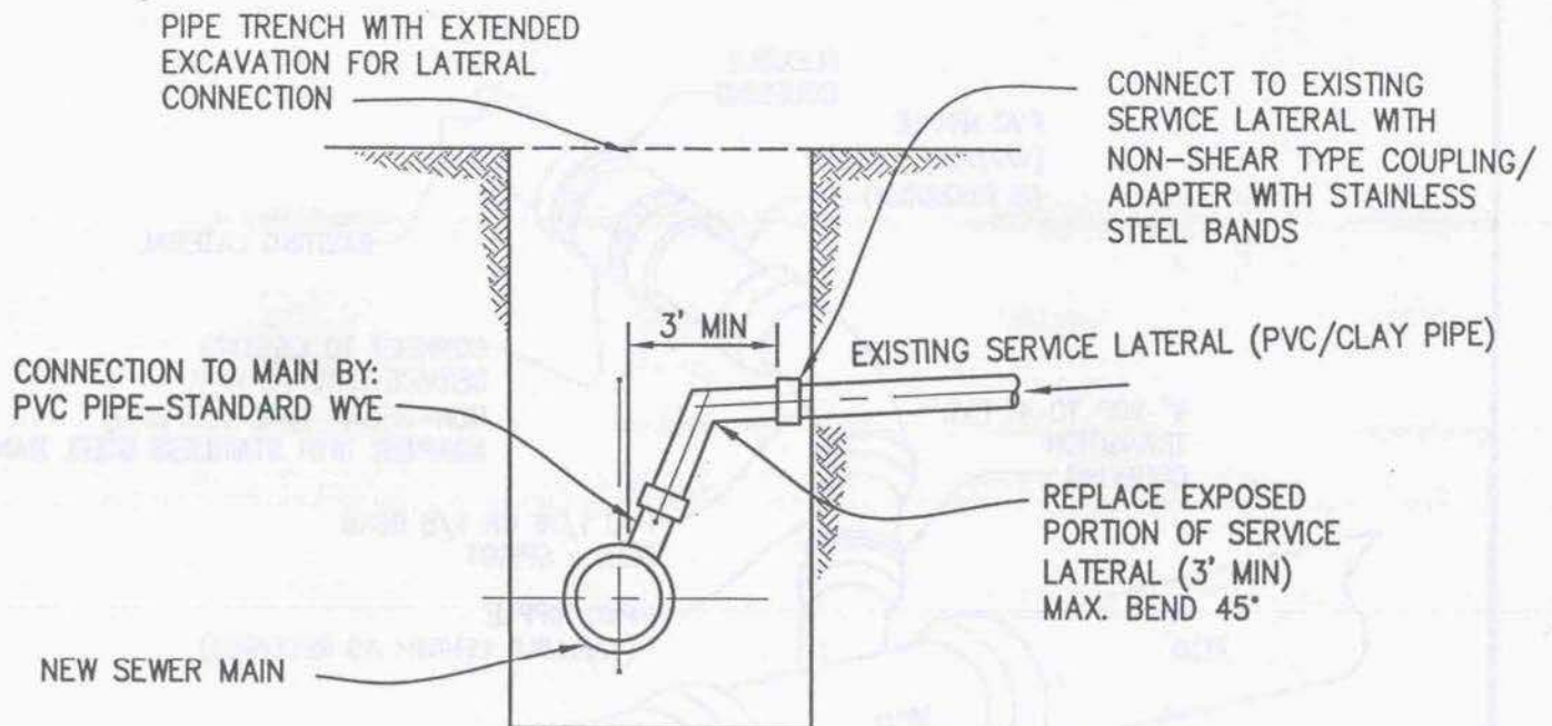
PVC PIPE LATERAL CONNECTION
